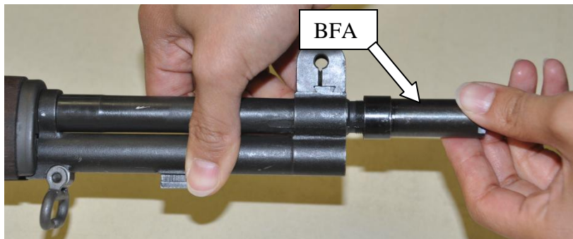
Figure 24. BFA removal
