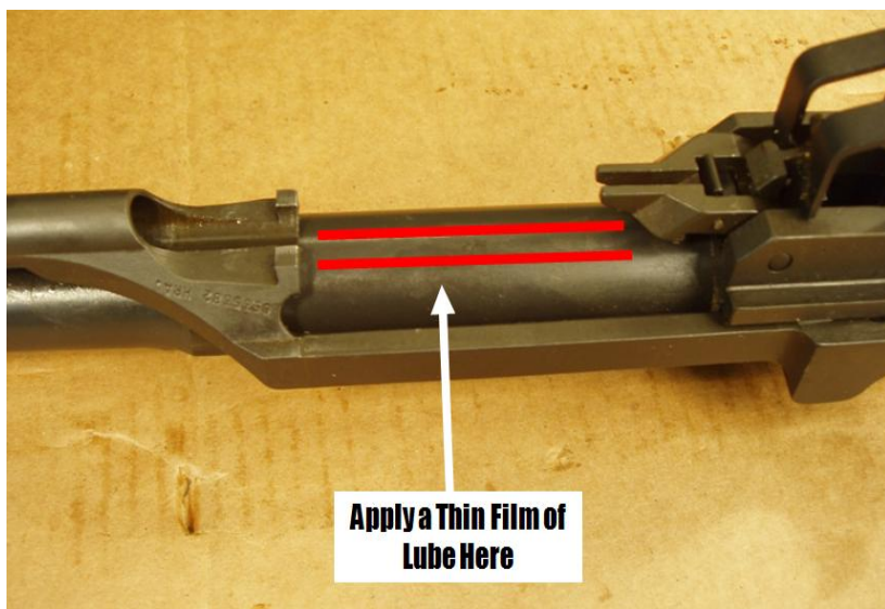
Figure 63. Lubrication
