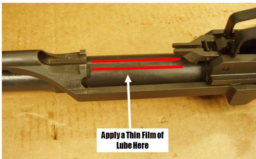
Figure 62. Lubrication
