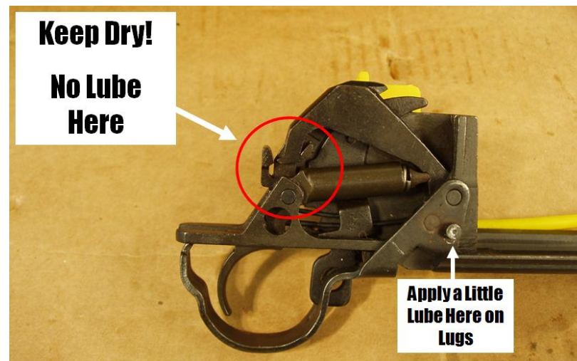
Figure 64. Lubrication
