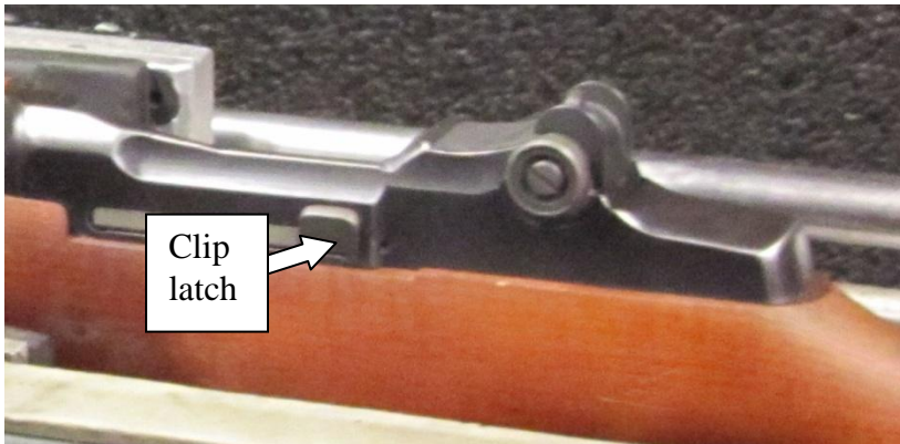
Figure 54. Clip latch
