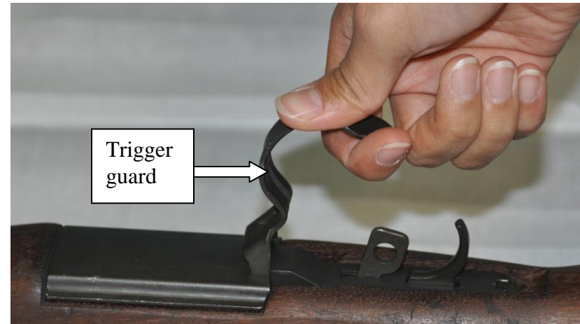
Figure 10. Trigger guard being pulled rearward and upward
